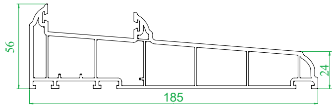
4006 185mm Cill
