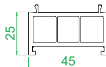
5025 25 mm Add on
