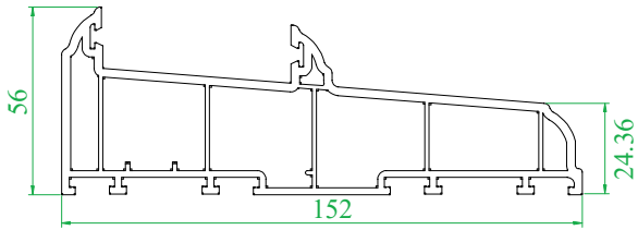
4005 150mm Cill
