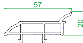
4013 Sash Stop with upstand
