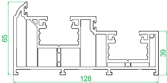
4001 Outer Frame
