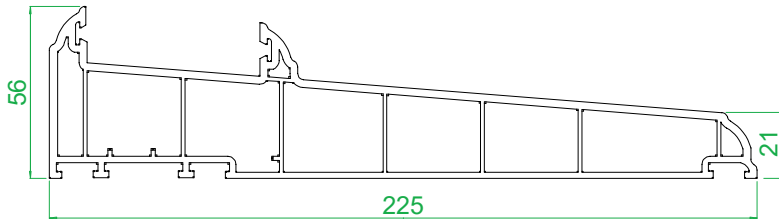
4007 225mm Cill
