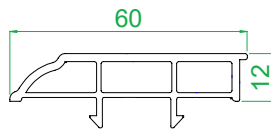
4012 Sash Stop
